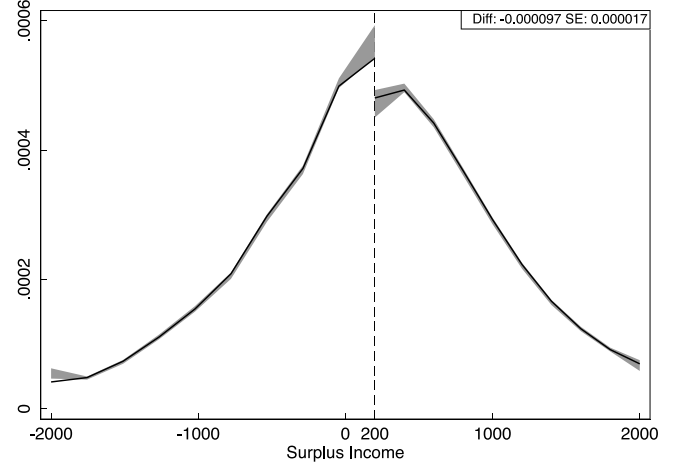
(b) Cattaneo et al. (2020) Test
